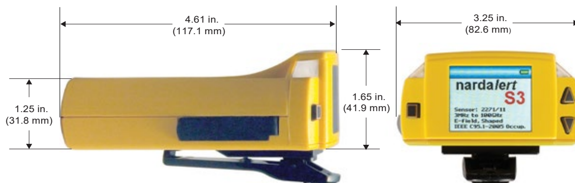
Fig. 7. Dimensions of the Nardalert S3 mainframe
